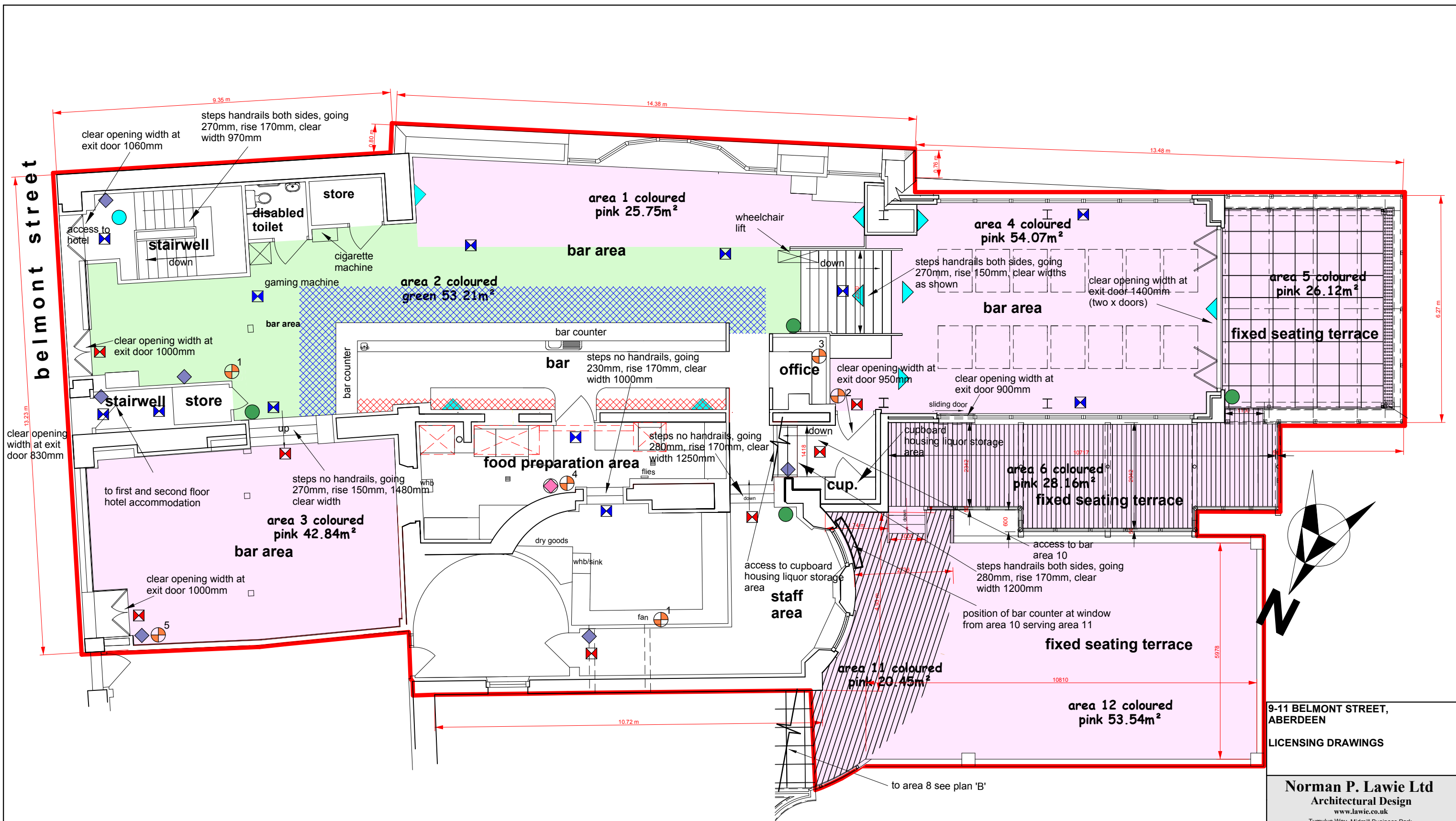
~ PART GROUND/LOWER GROUND FLOOR LAYOUT ~ PLAN 'D'
